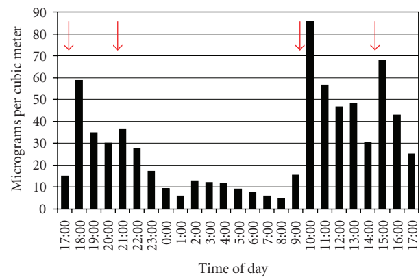
FIGURE 5: Representative display of PM 2.5 concentration hourly averages over a twenty-four hour sampling period in one home (site Nav135). On the basis of interviews with residents, spikes in PM 2.5 concentrations coincided with activities such as adding chunks of coal to the stove (red arrows).
